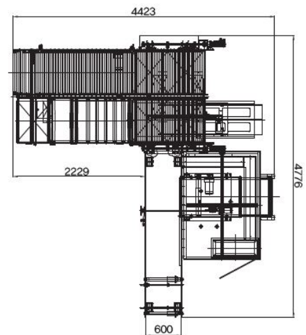
L-Shape Configuration
